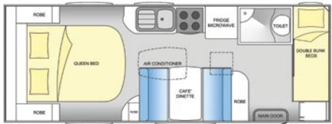
Alternative layout option: L shape dinette and triple bunk beds.
